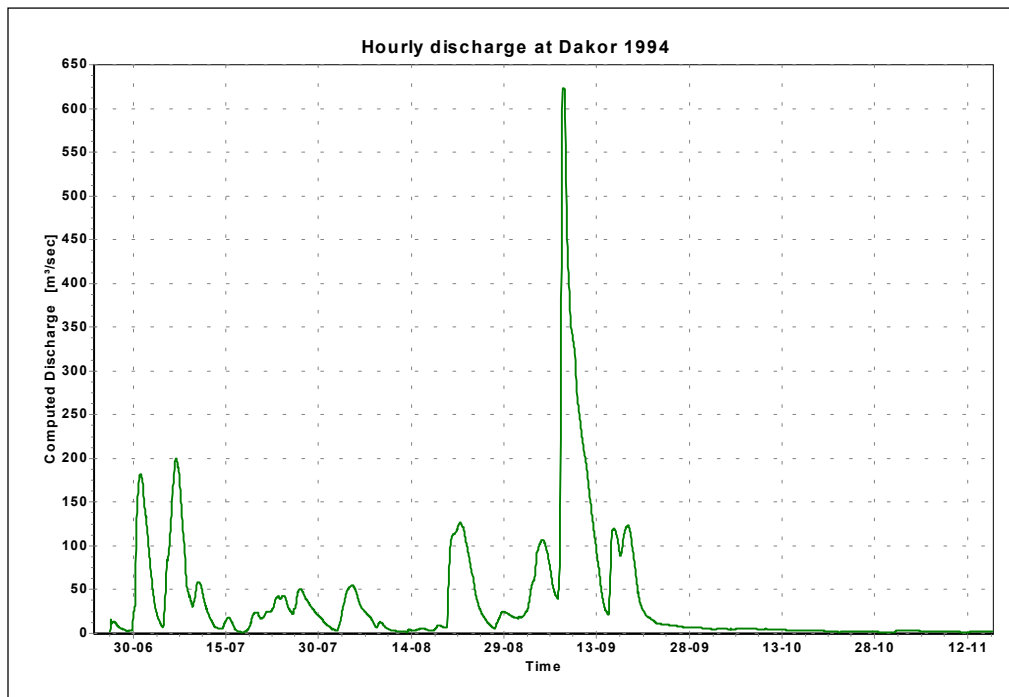
Figure 10: Hourly runoff at Dakor for 1994
