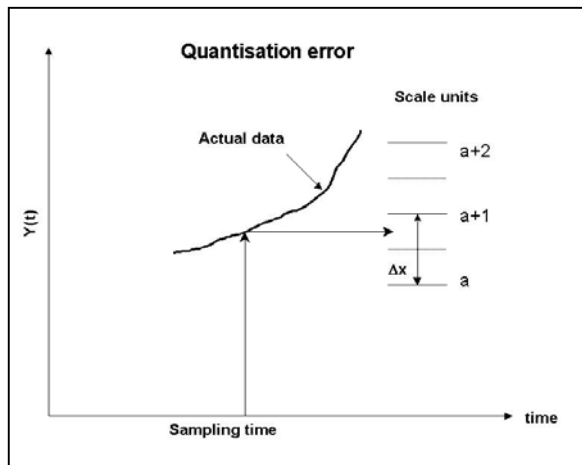
Figure 4.2: Quantisation error
